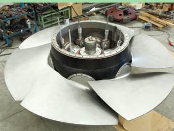
Fabrication of Kaplan runner Complete assembly, ready for erection
